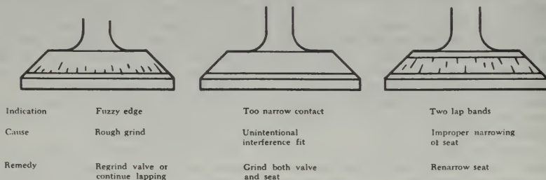
FIGURE 10-19. Incorrectly lapped valves.
